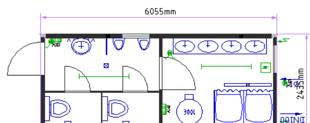
Sanitary cabin 20'
