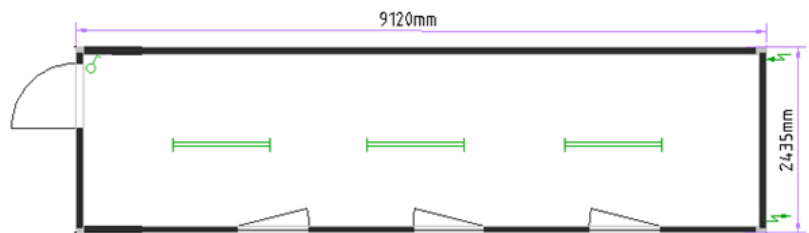
Portable cabin 30'
