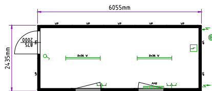
Portable cabin 20' standard
