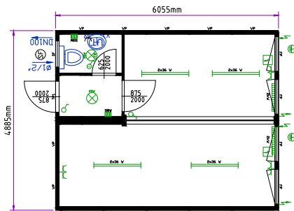
Portable and sanitary cabin 2 units
