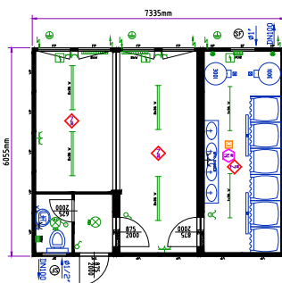
Portable and sanitary cabin 3 units
